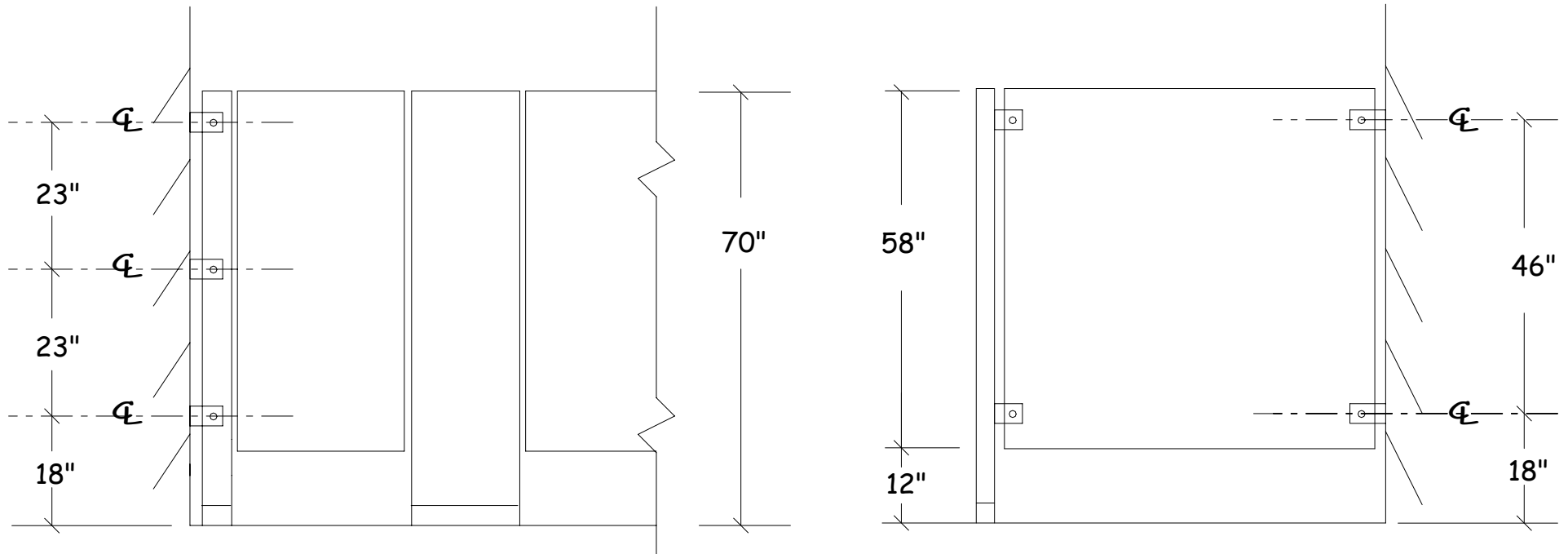
Series FM - Typical elevation
