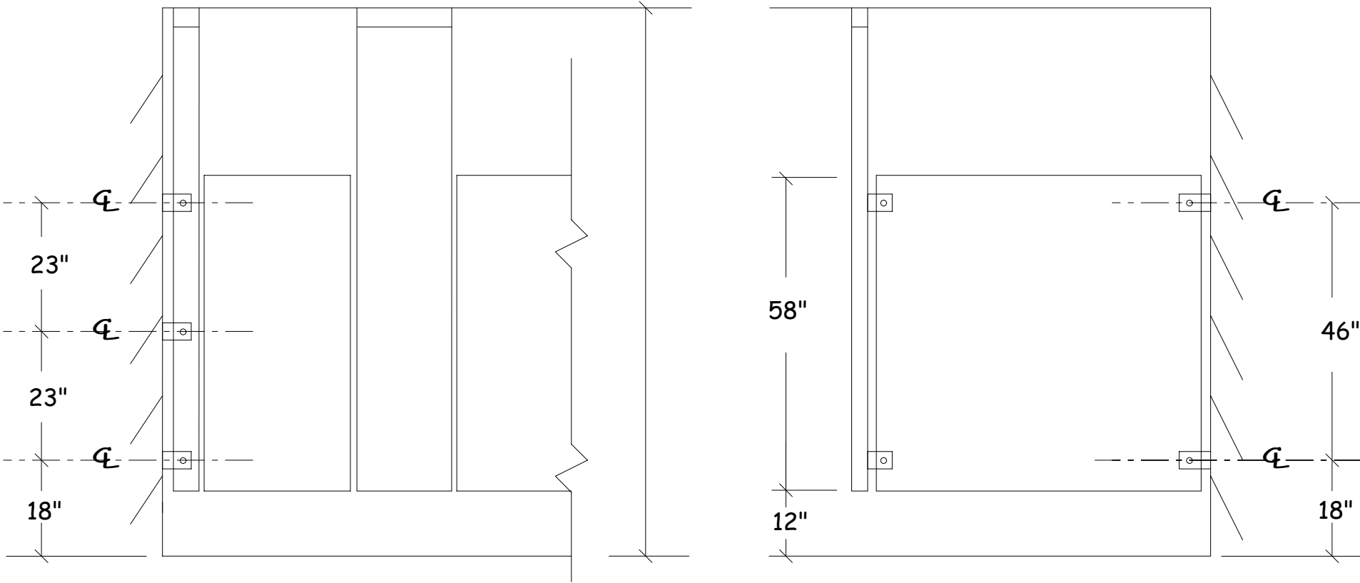
Series CH - Typical elevation
