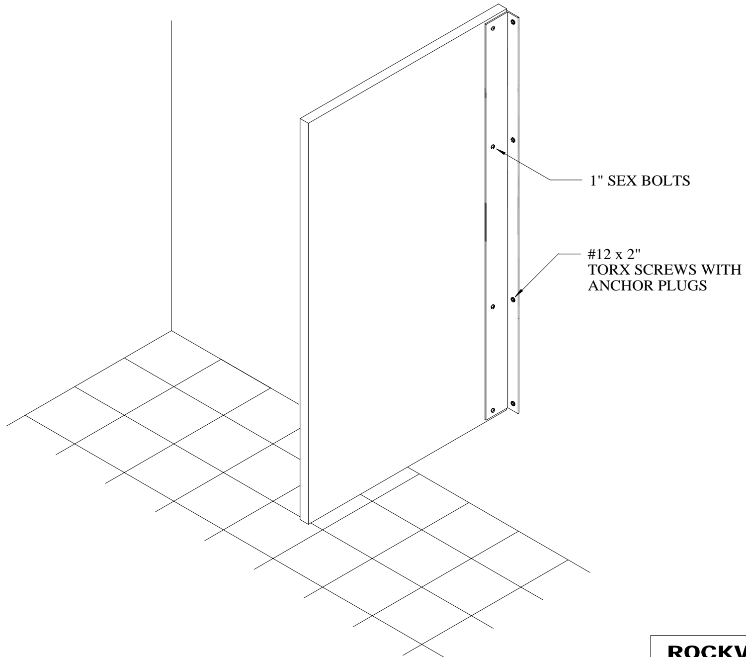
WHF-6 URINAL SCREEN DETAIL
