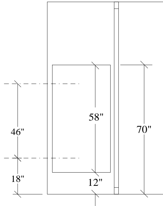
BACKING LOCATIONS
