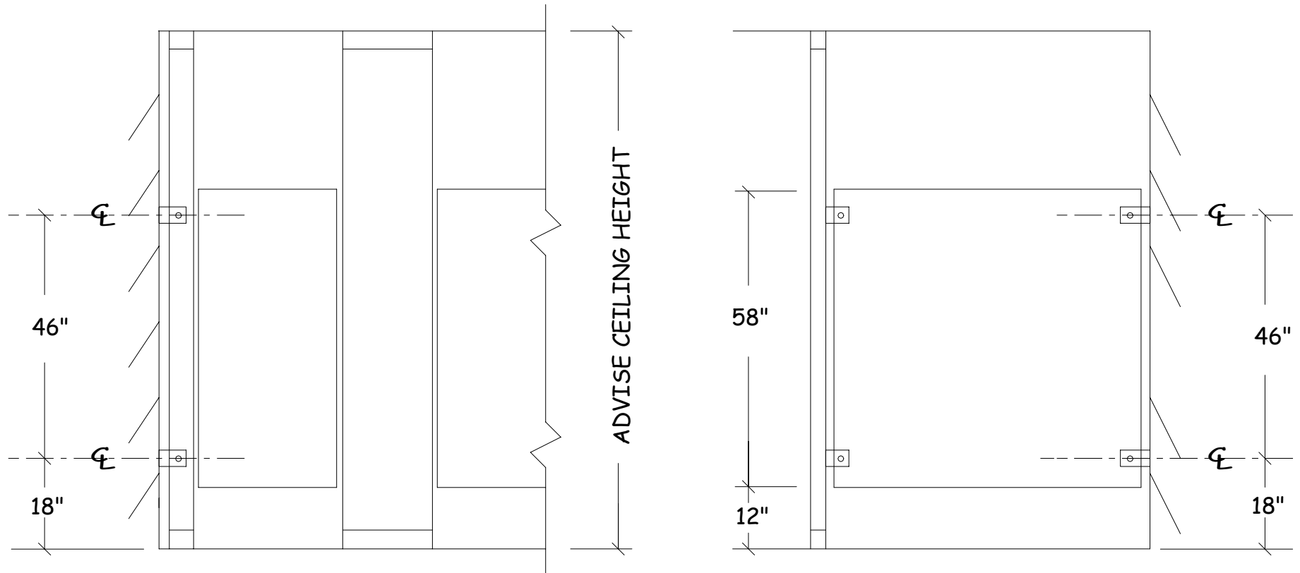
Series FC - Typical elevation Backing points for other than masonry walls indicated
