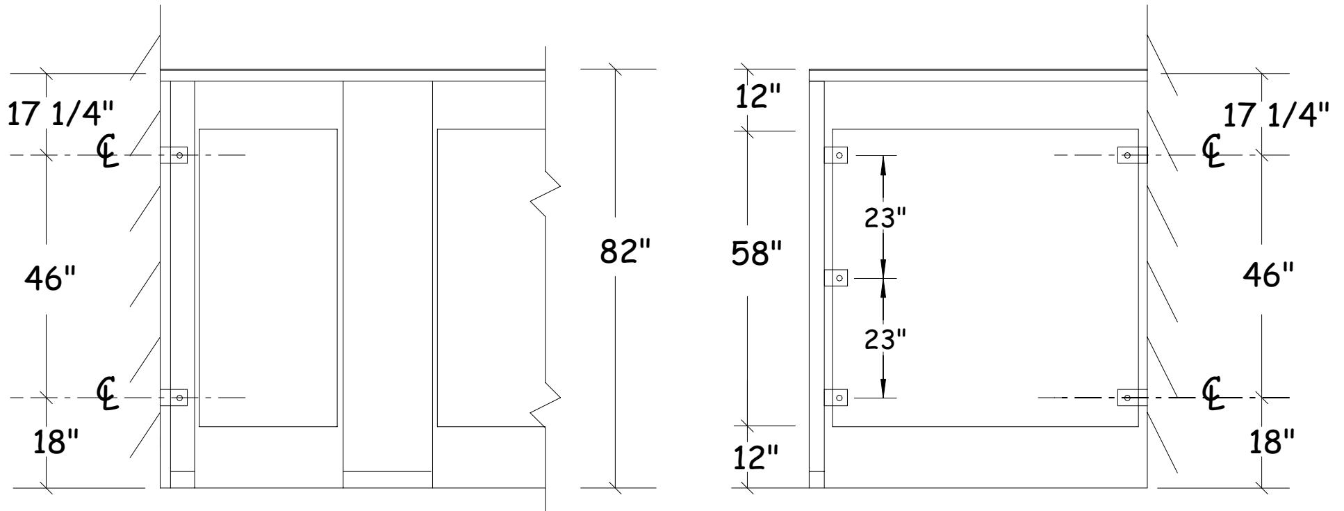
Series OH - Typical elevation Backing points for other than masonry walls indicated
