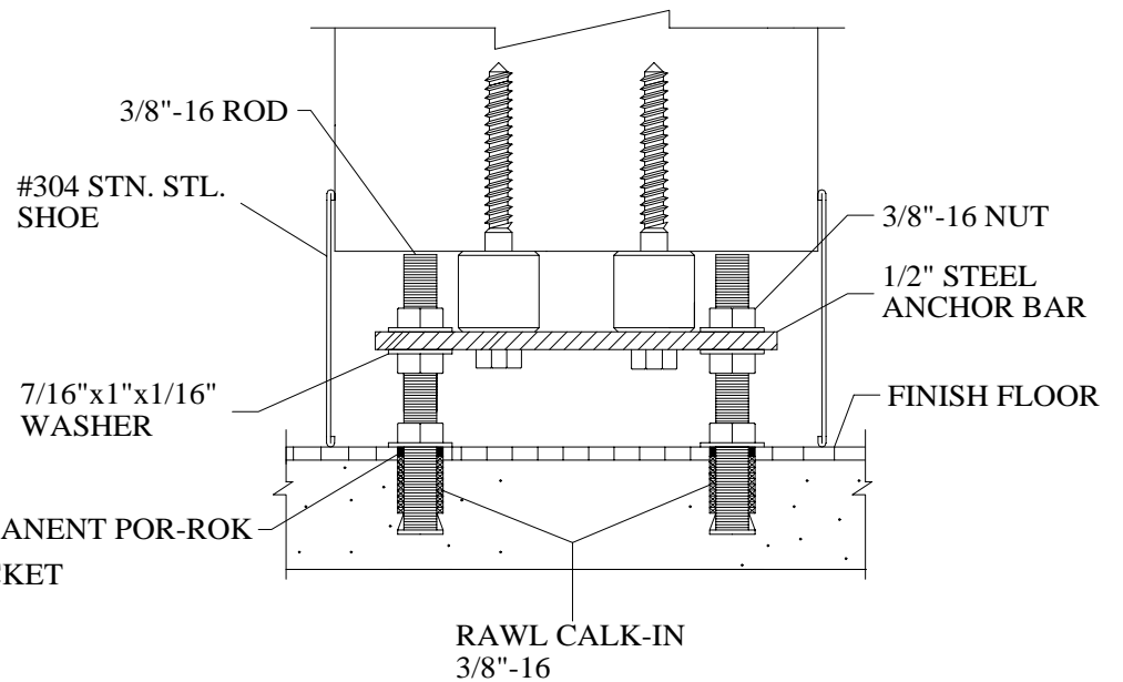
FM-4 FLOOR CONNECTION
